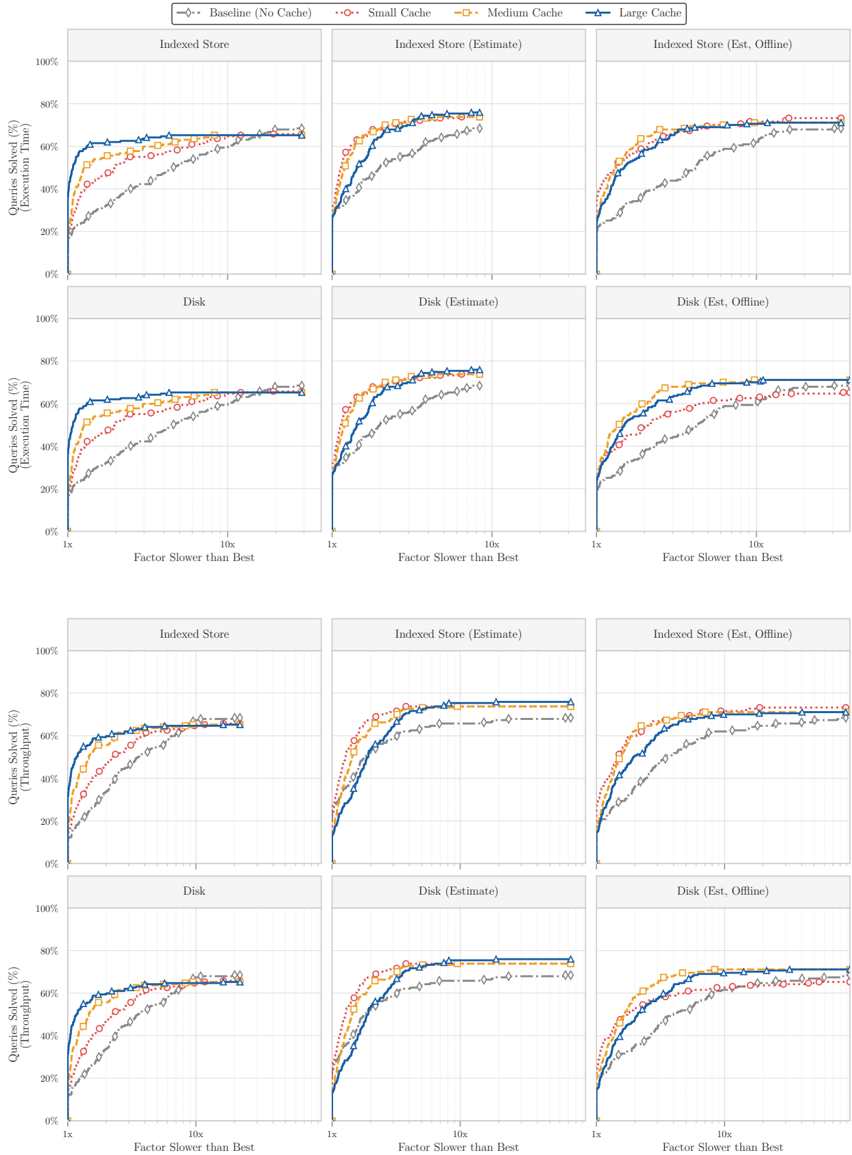
Figure 3: Performance profiles of the in-memory and disk-based quad store caches families of algorithms. The y-axis shows the percentage of queries executing within a factor (x-axis) of the fastest algorithm.
