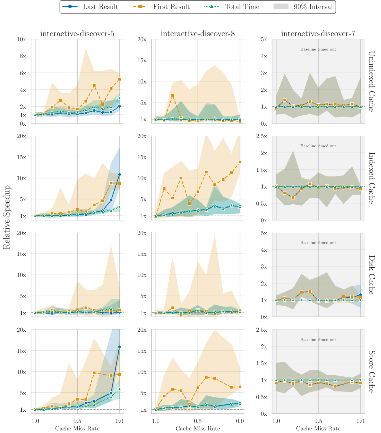
Figure 7: Performance of unindexed, LRU indexed, In-memory store, and Disk-based store caches across representative query templates. The y-axis shows the mean speedup relative to a baseline with a 0% hit rate. Shaded regions denote the 90th percentile {TODO: Placeholder disk figure}
