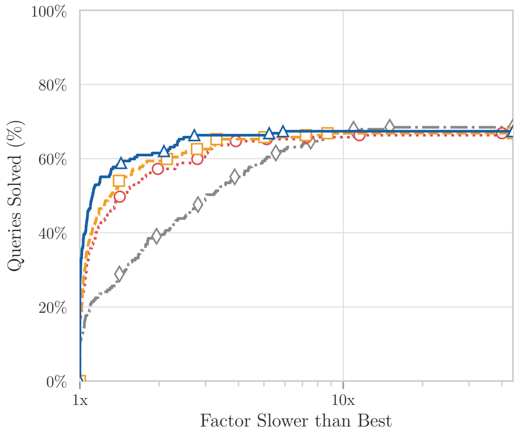
Unindexed Cache (Throughput)
