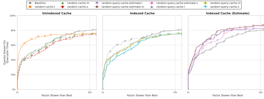
Fig. 6. Performance profile of the tested cache algorithms on random query sequences. The y-axis shows the percentage of queries that execute within a given performance factor (x-axis) of the fastest algorithm for that query.
