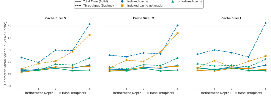
Fig. 3. Geometric mean of observed speedups and increases respectively for total execution time and query throughput relative to the no caching baseline across refinement depths.
