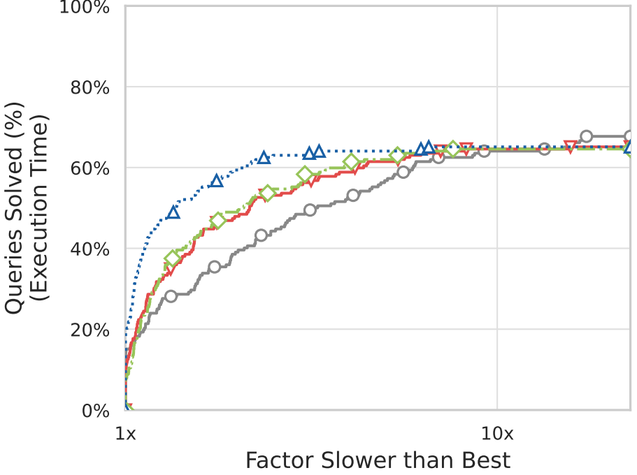
Unindexed Cache
