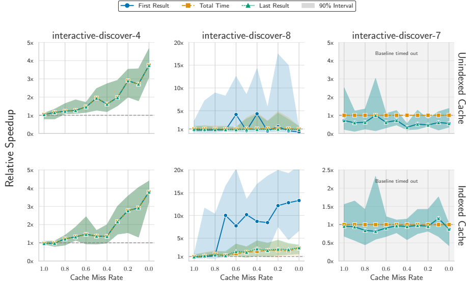
Fig. 4. Performance of unindexed and indexed caches across representative query templates. The y-axis shows the mean speedup relative to a baseline with a 0% hit rate. Shaded regions denote the 90th percentile
