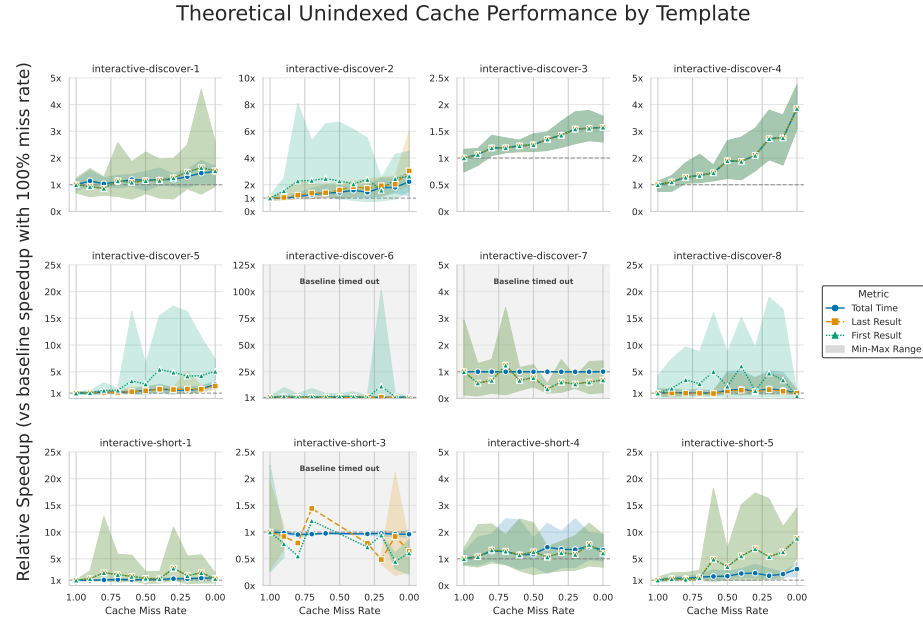
Fig. 3. Theoretical unindexed cache performance by query template. Lines indicate the mean relative speedup of the repeated query for total execution time, first result, and last result against a 100% miss rate baseline. Shaded regions denote the absolute minimum and maximum variance across iterations.
