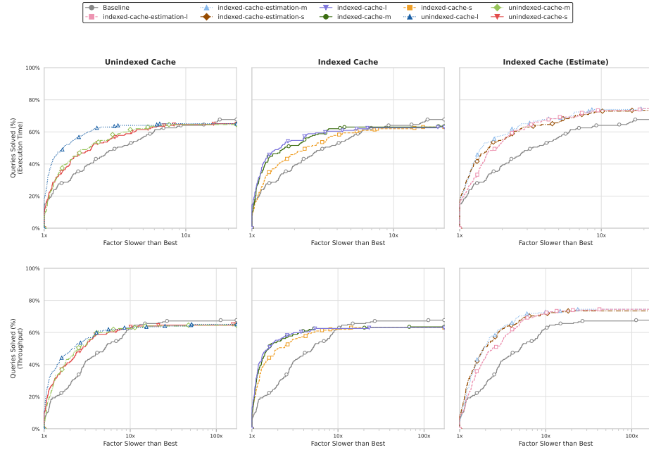
Fig. 1. Performance profile of the tested cache algorithms. The y-axis shows the percentage of queries that execute within a given performance factor (x-axis) of the fastest algorithm for that query.
