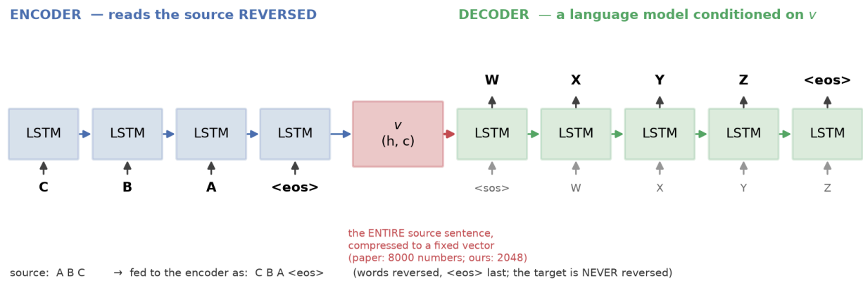
Sequence-to-sequence with a reversed source (Sutskever et al., 2014, Fig. 1)
