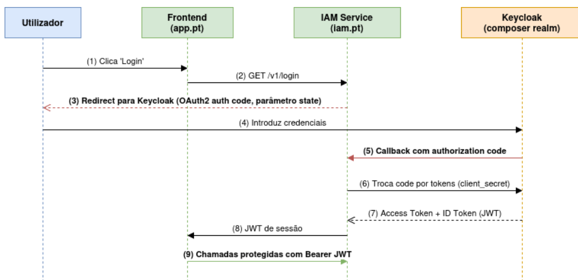
Figura 3: Fluxo de Login OIDC (OAuth2 Authorization Code Flow)
