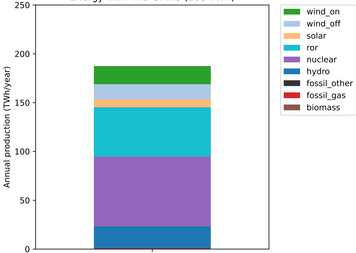
Energy mix - MD SMR6 (208 TWh)
