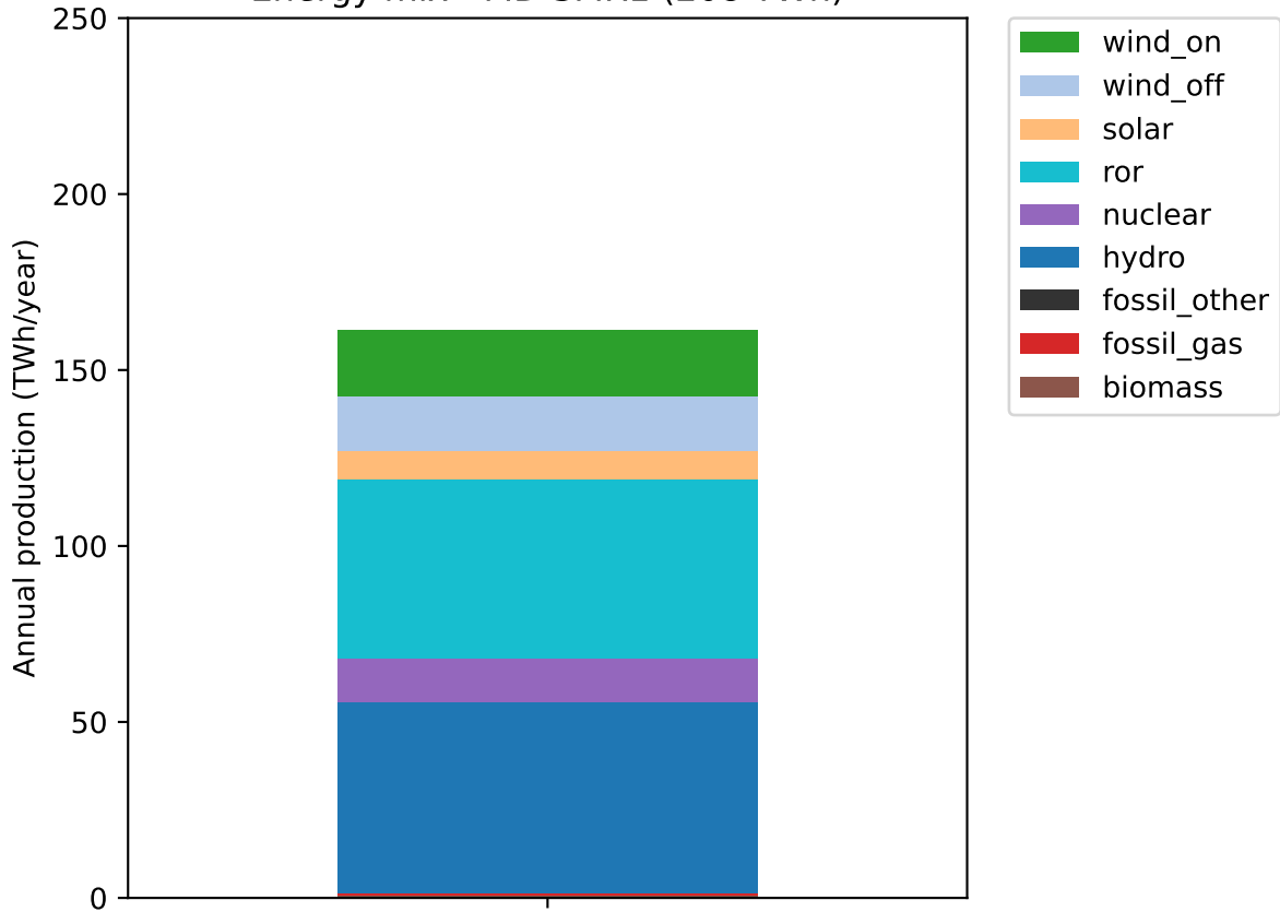
Energy mix - MD SMR1 (208 TWh)
