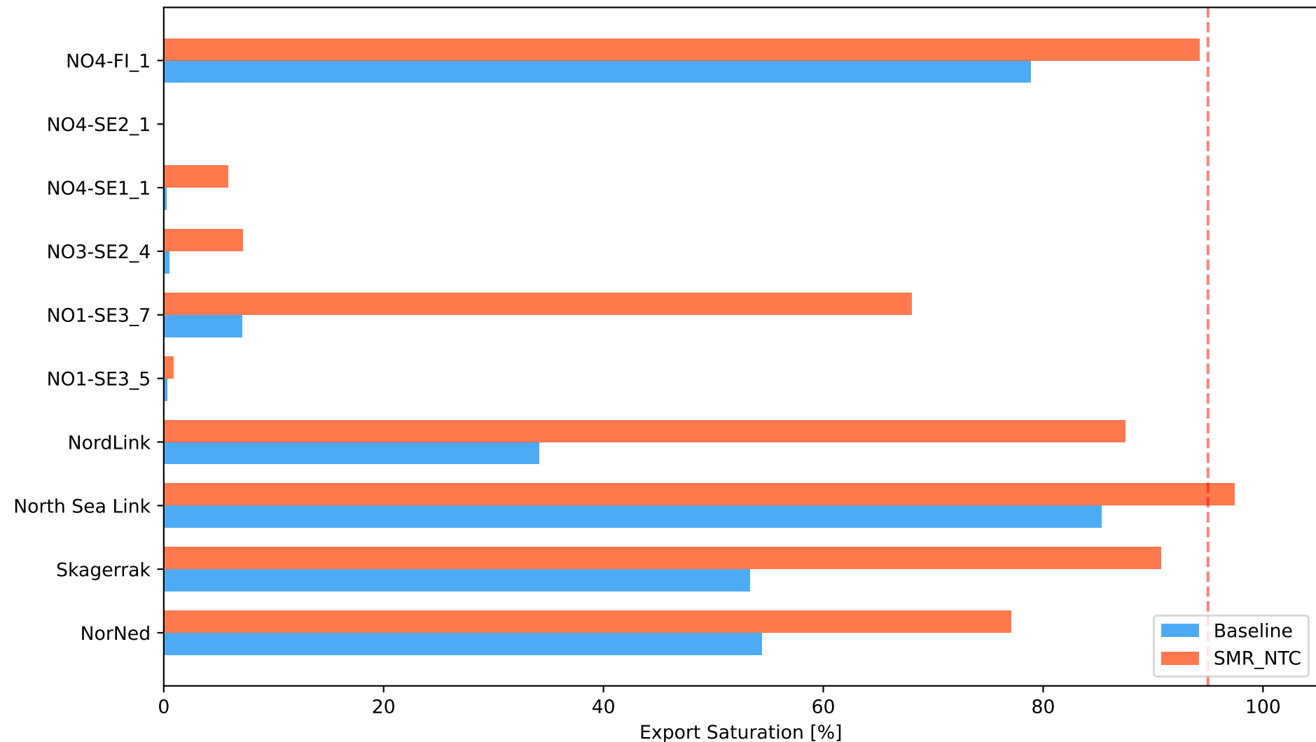
Cable Saturation (>95% NTC) — MD Demand
