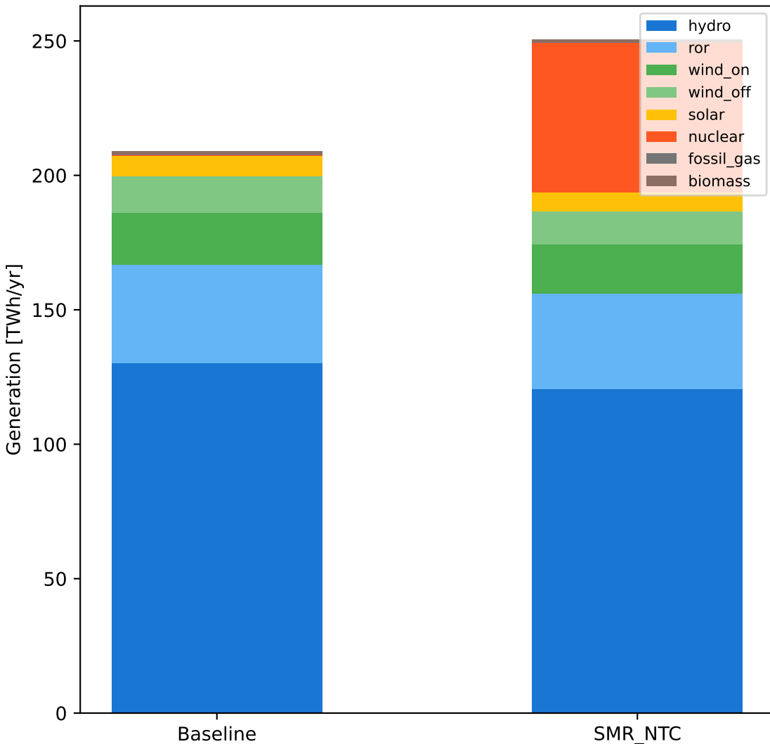
Norway Generation Mix — MD Demand
