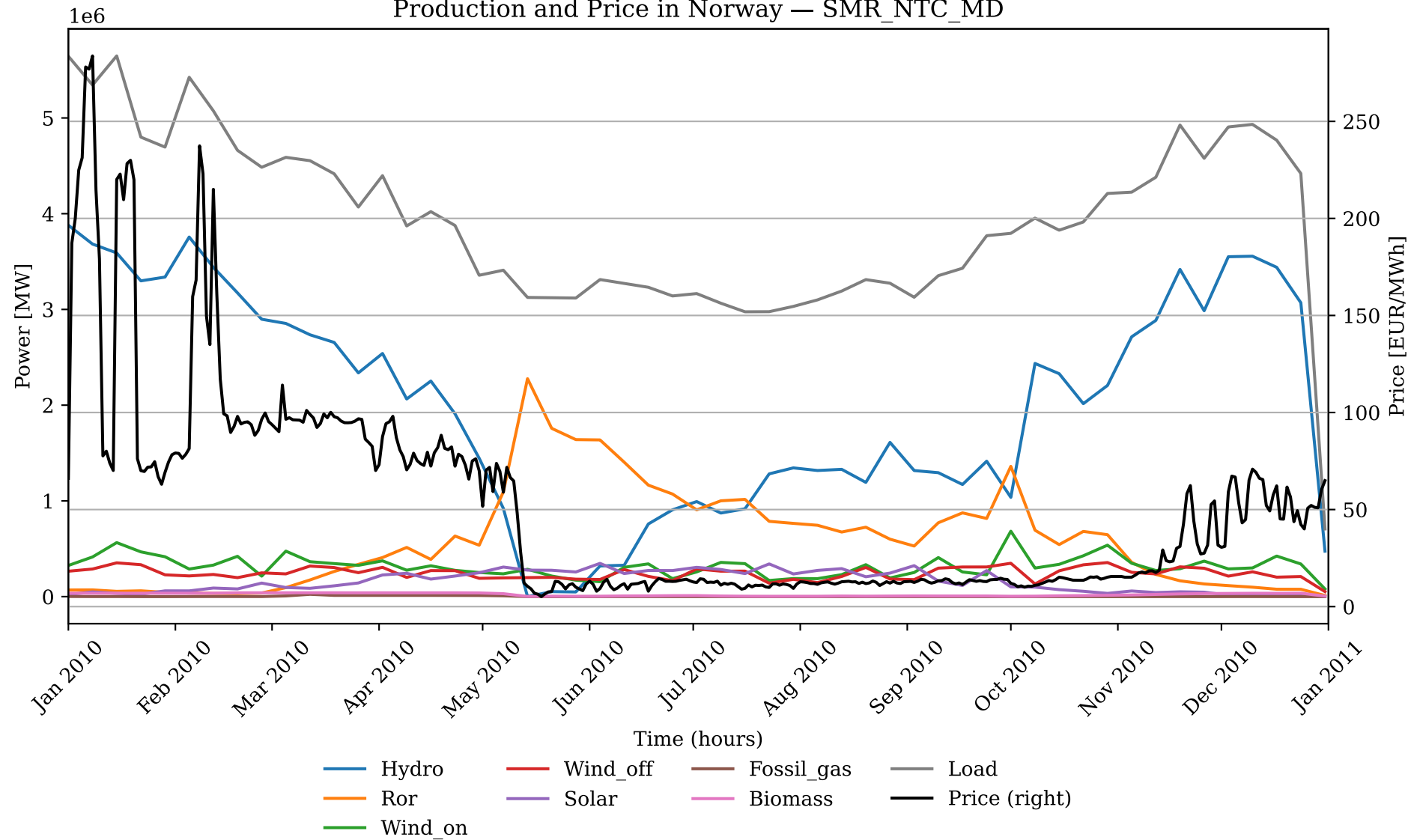
Production and Price in Norway — SMR_NTC_MD
