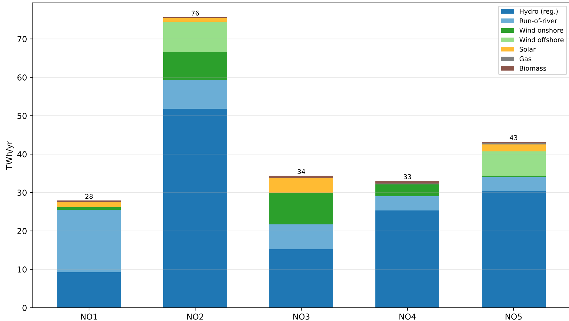
IC BL (0 GW) — Generation Mix per Zone (annual avg)
