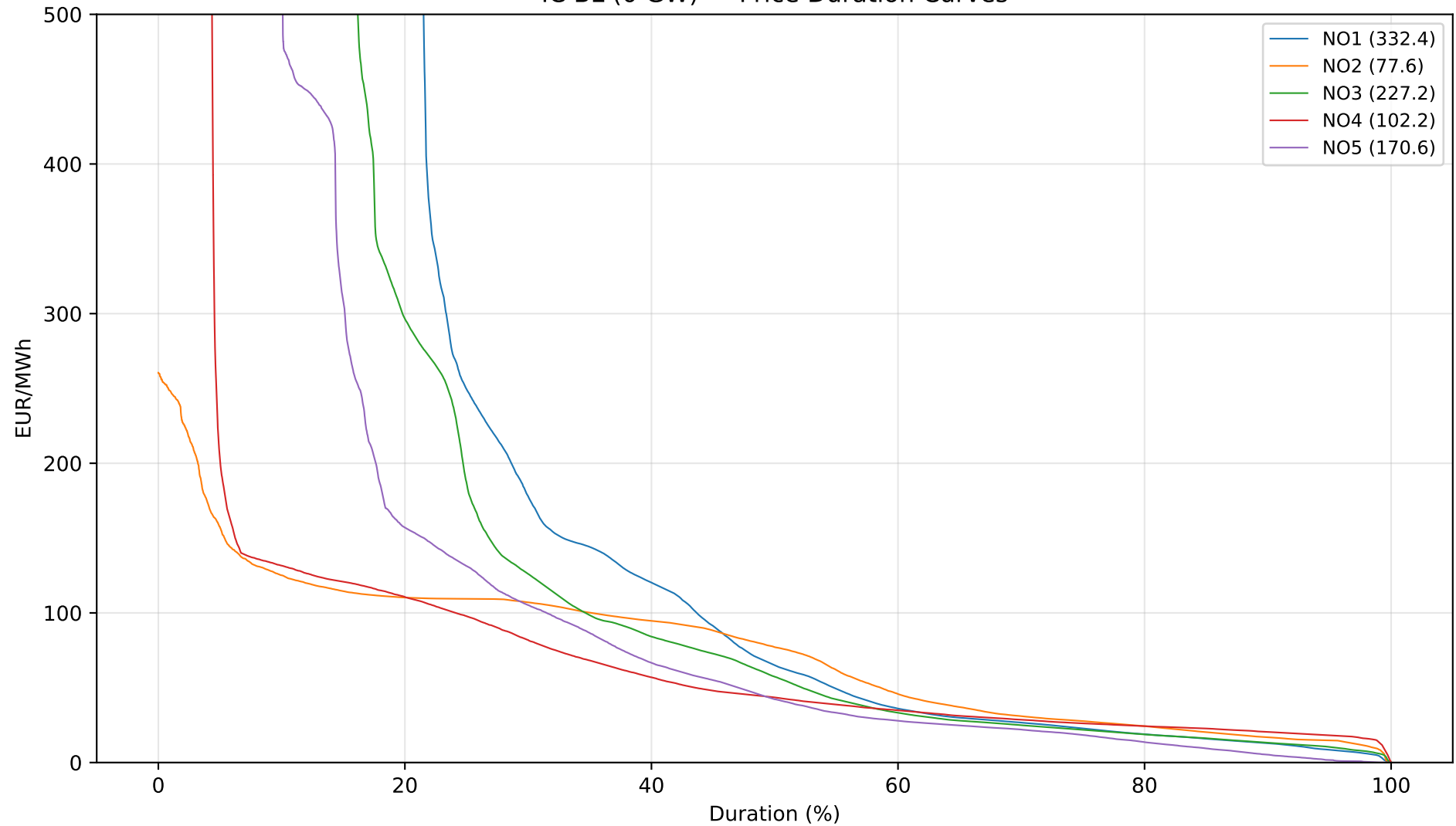
IC BL (0 GW) — Price Duration Curves
