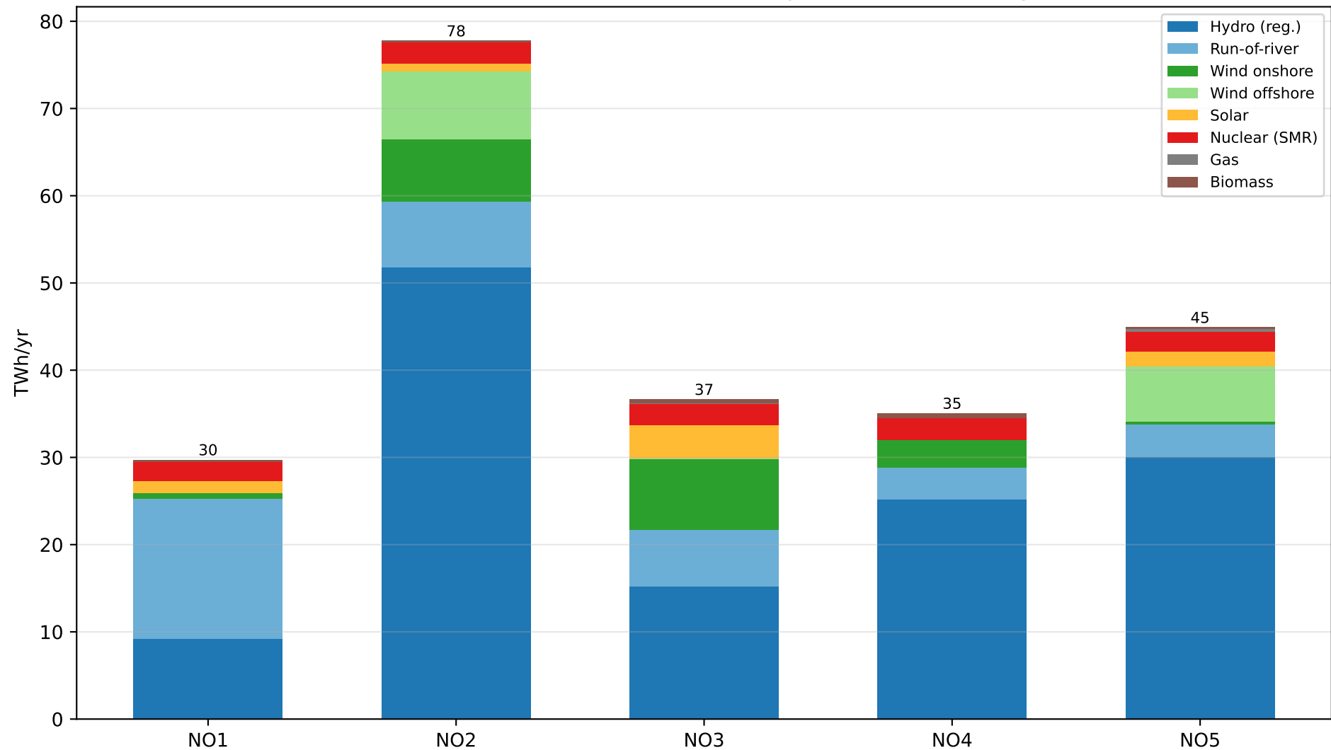
IC SMR1 (1.5 GW) — Generation Mix per Zone (annual avg)
