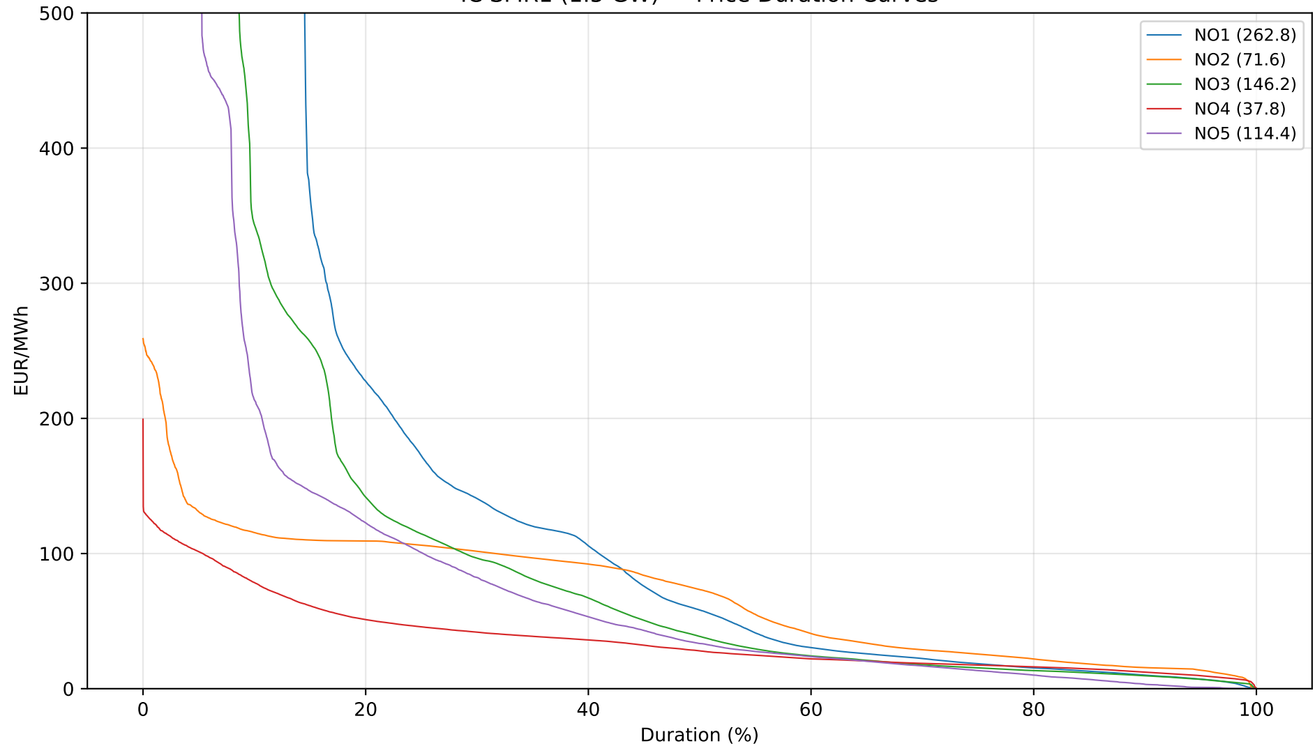
IC SMR1 (1.5 GW) — Price Duration Curves
