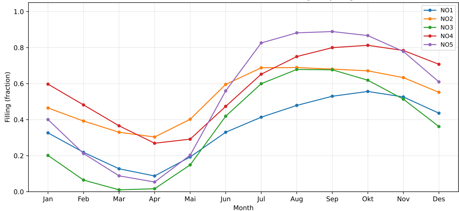
IC SMR1 (1.5 GW) — Seasonal Reservoir Filling (30-yr avg)
