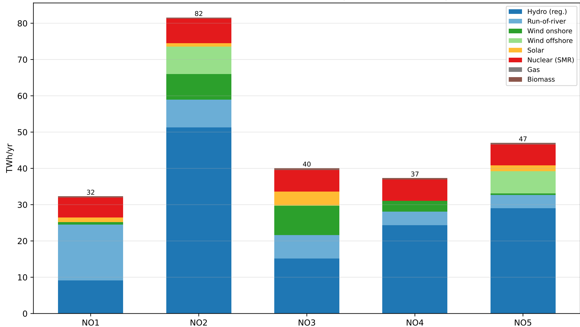
IC SMR3 (4.5 GW) — Generation Mix per Zone (annual avg)
