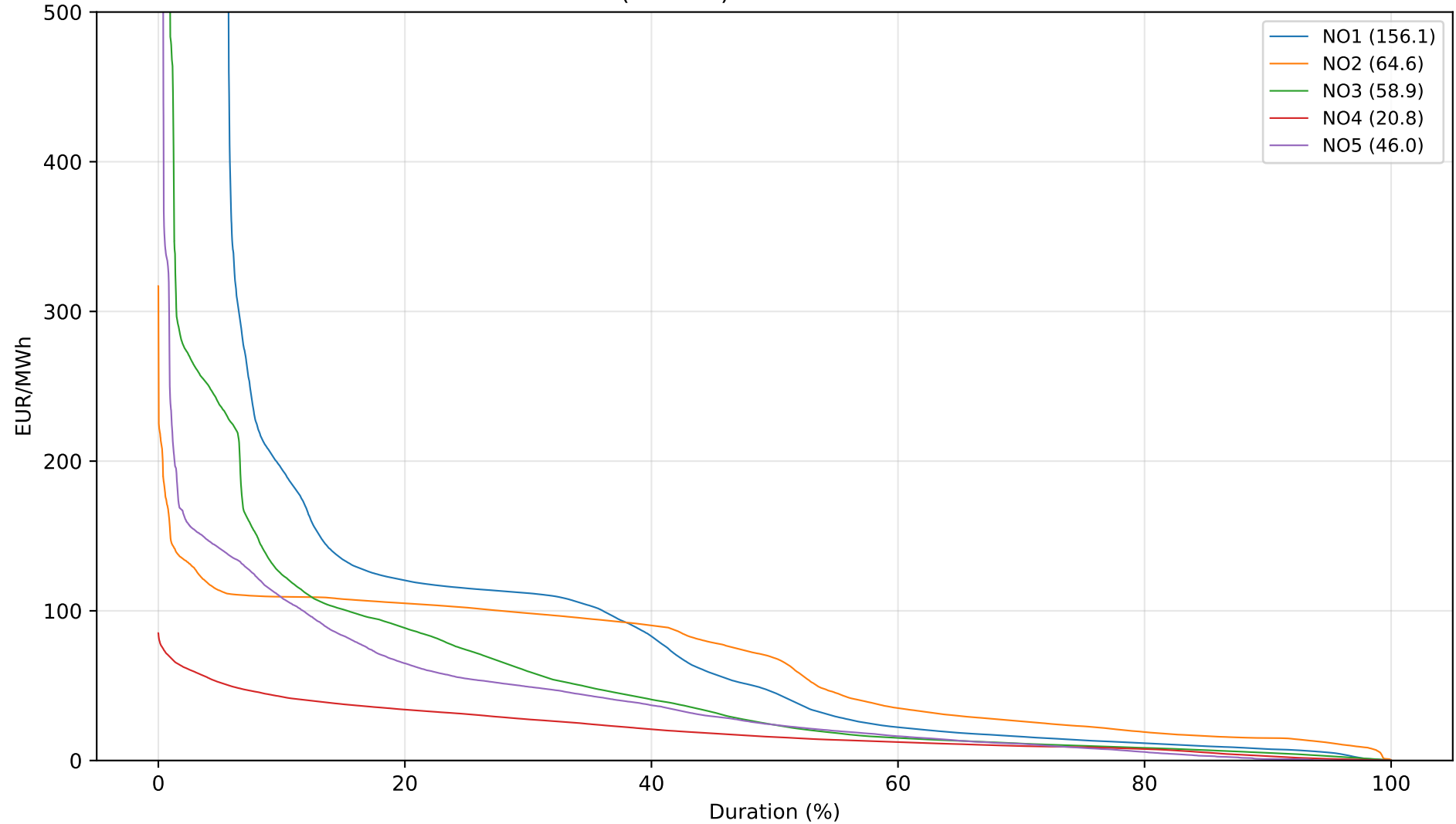
IC SMR3 (4.5 GW) — Price Duration Curves
