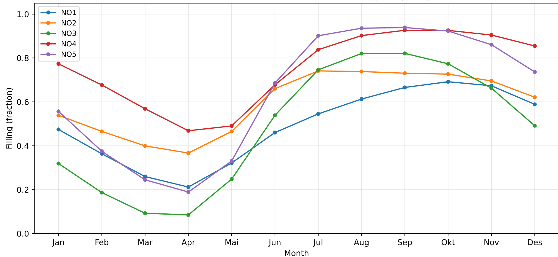
IC SMR3 (4.5 GW) — Seasonal Reservoir Filling (30-yr avg)
