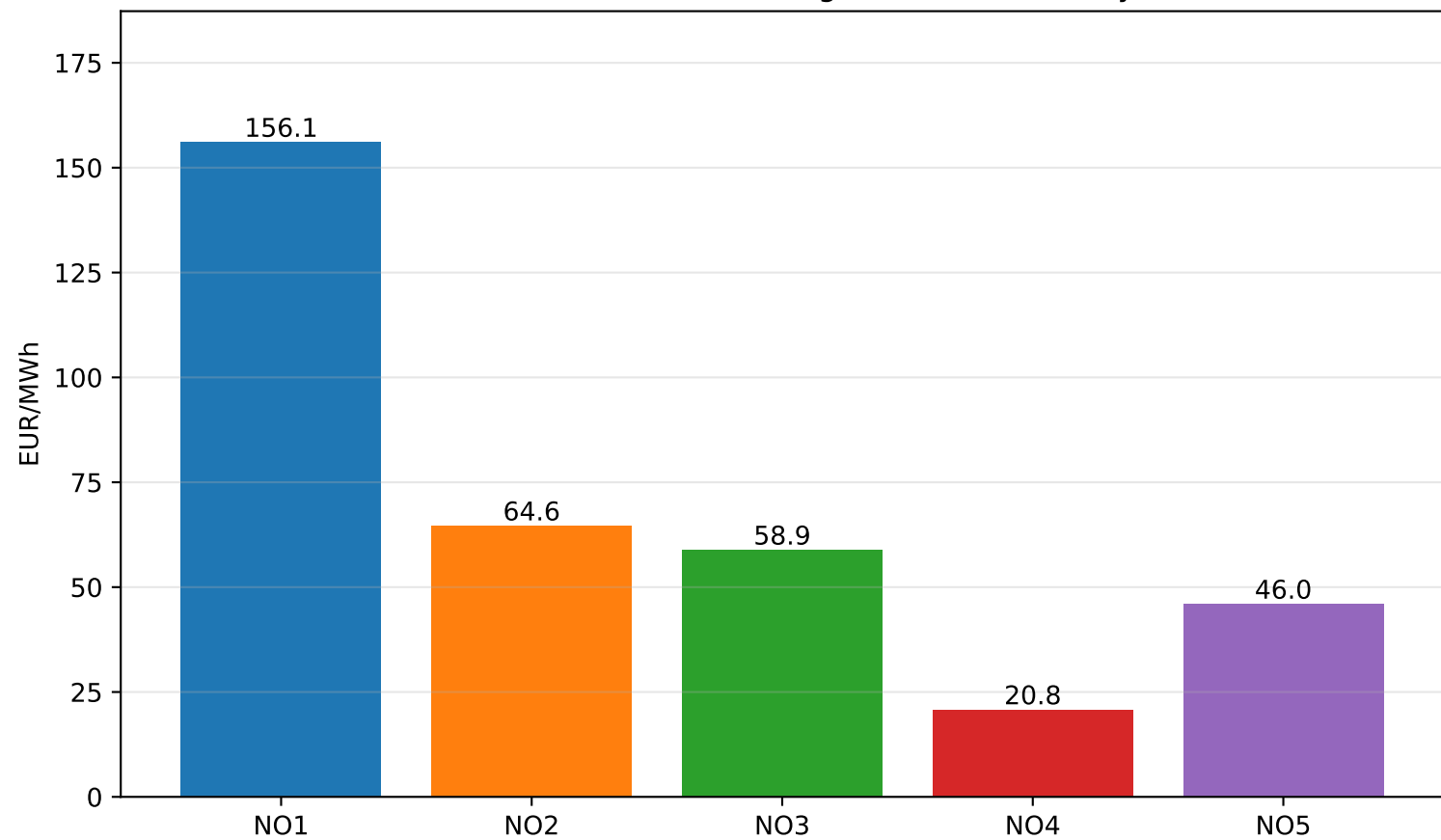
IC SMR3 (4.5 GW) — Average Zone Prices (30-yr)
