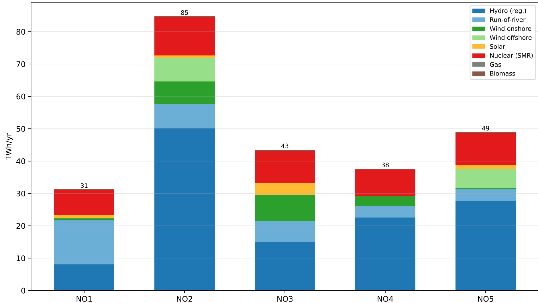
IC SMR6 (9.0 GW) — Generation Mix per Zone (annual avg)
