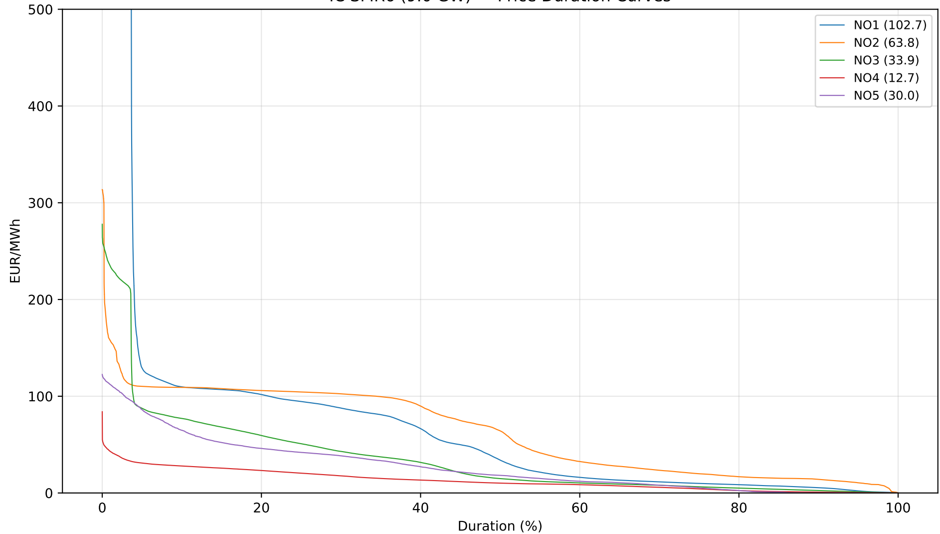
IC SMR6 (9.0 GW) — Price Duration Curves
