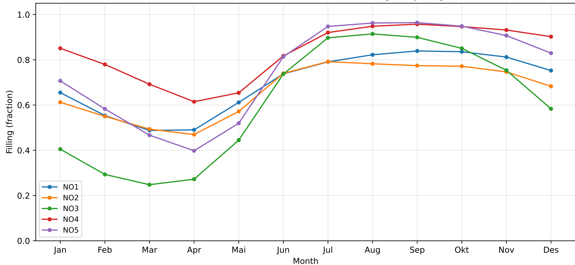
IC SMR6 (9.0 GW) — Seasonal Reservoir Filling (30-yr avg)
