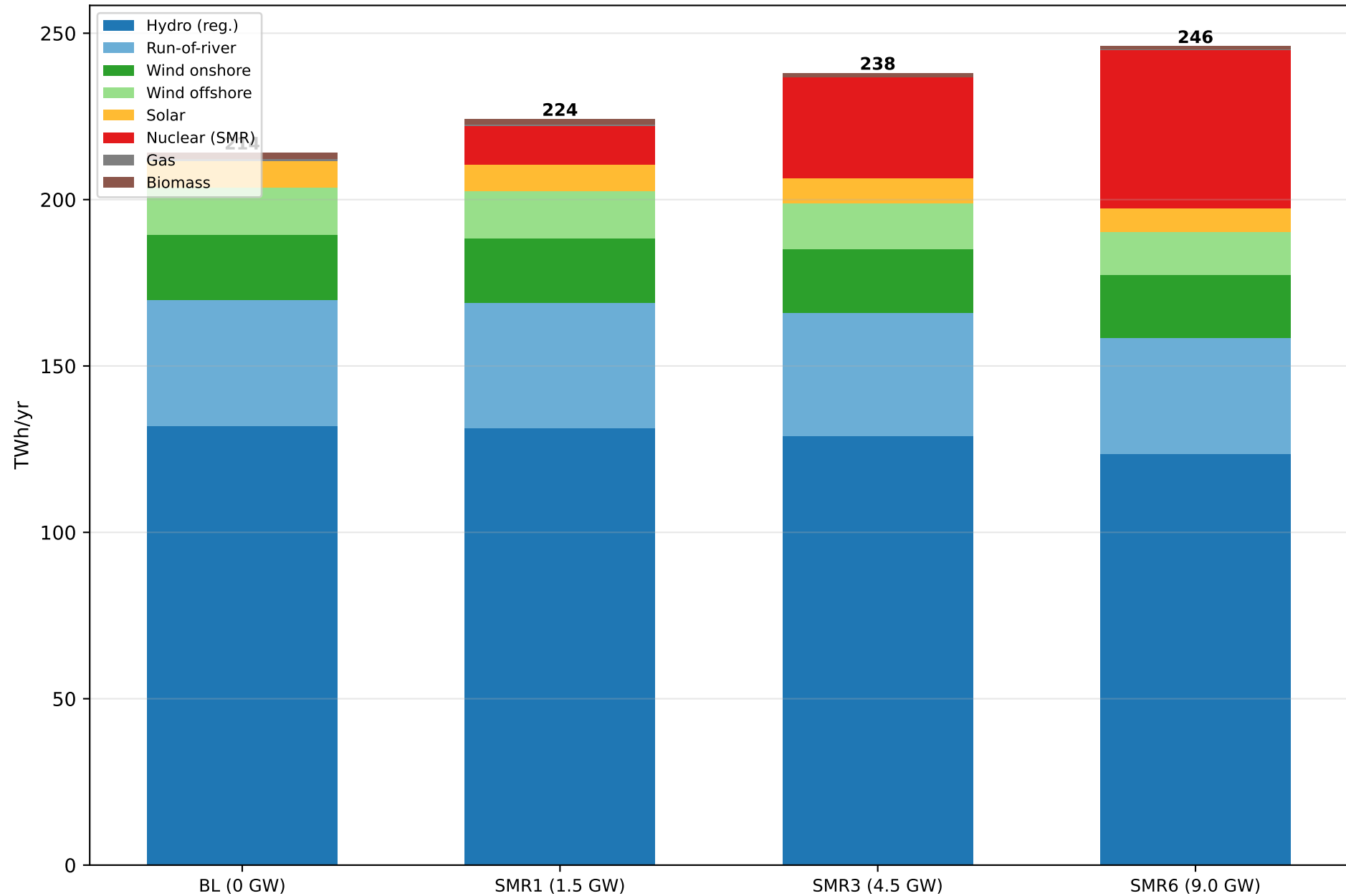
Norway Generation Mix — IC Nuclear Scenarios (annual avg, 230 TWh)
