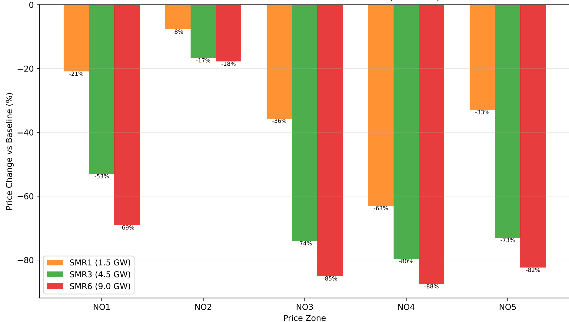
Price Reduction from Nuclear — IC Scenarios (230 TWh)
