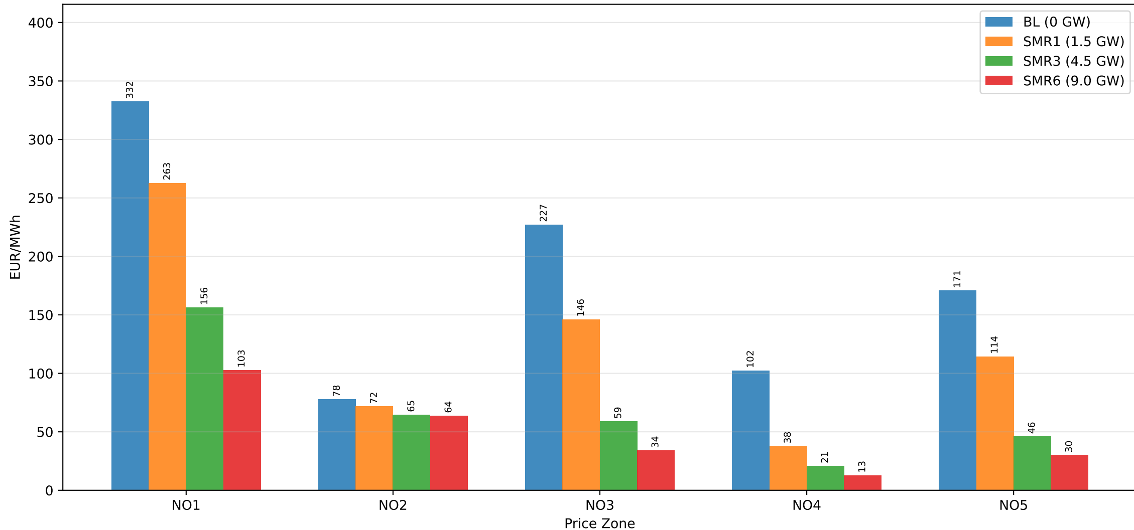
Zone Prices — IC Nuclear Scenarios (30-year average, 230 TWh)
