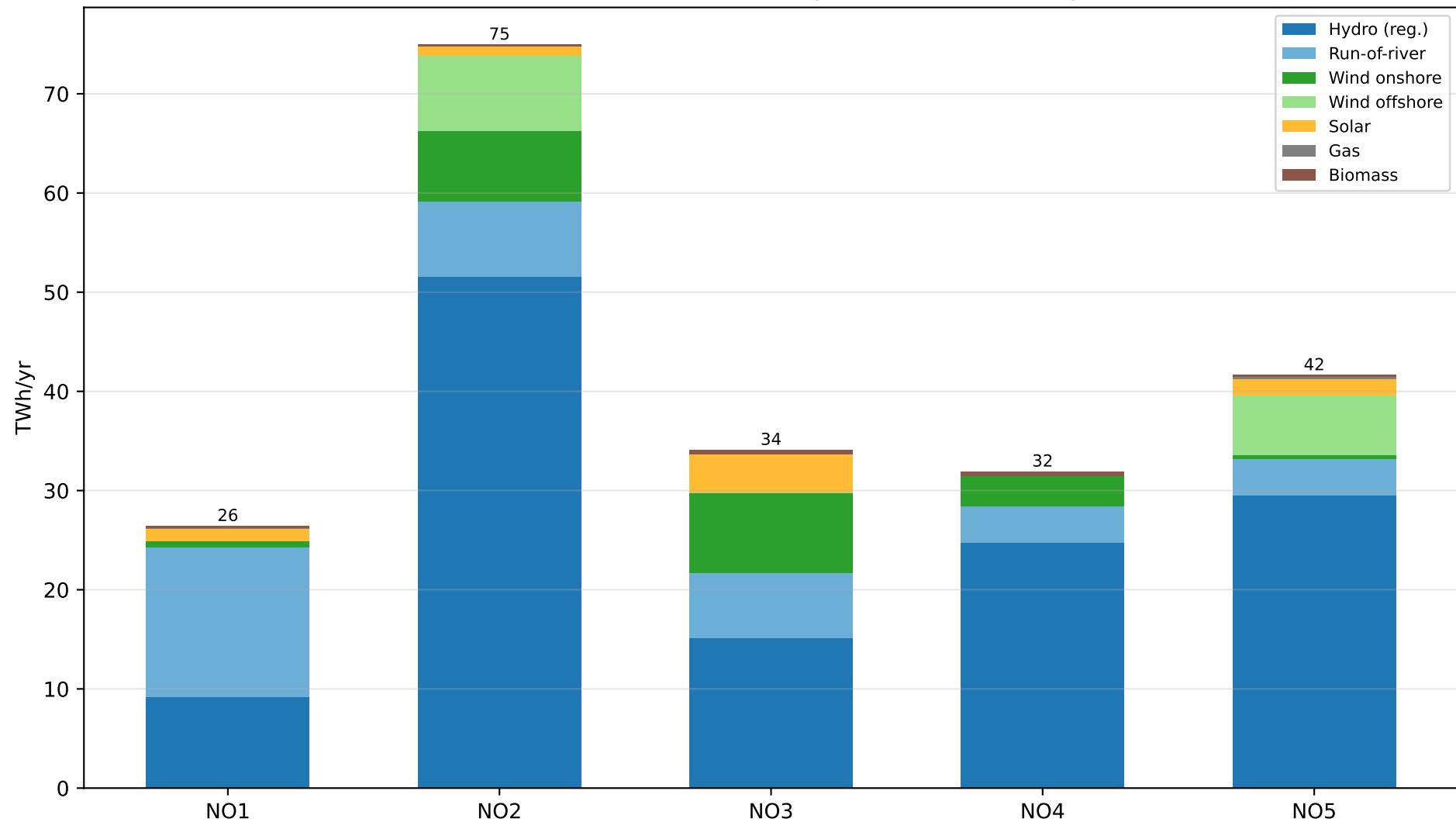
BL (0 GW) — Generation Mix per Zone (annual avg)
