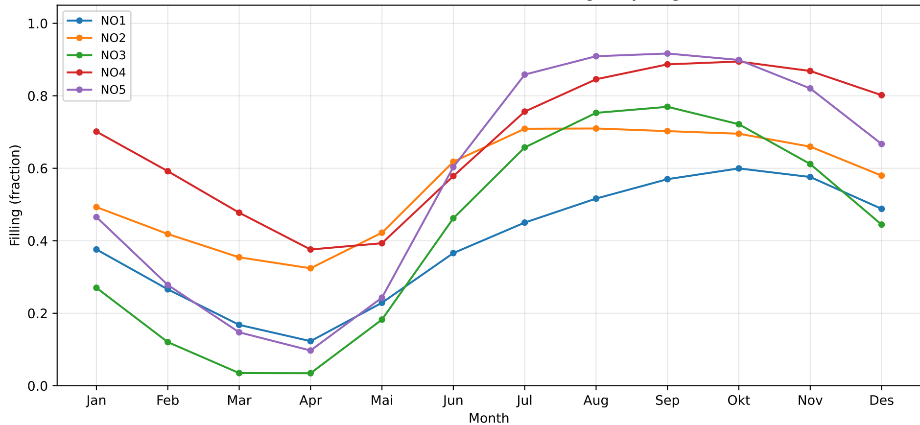
BL (0 GW) — Seasonal Reservoir Filling (30-yr avg)
