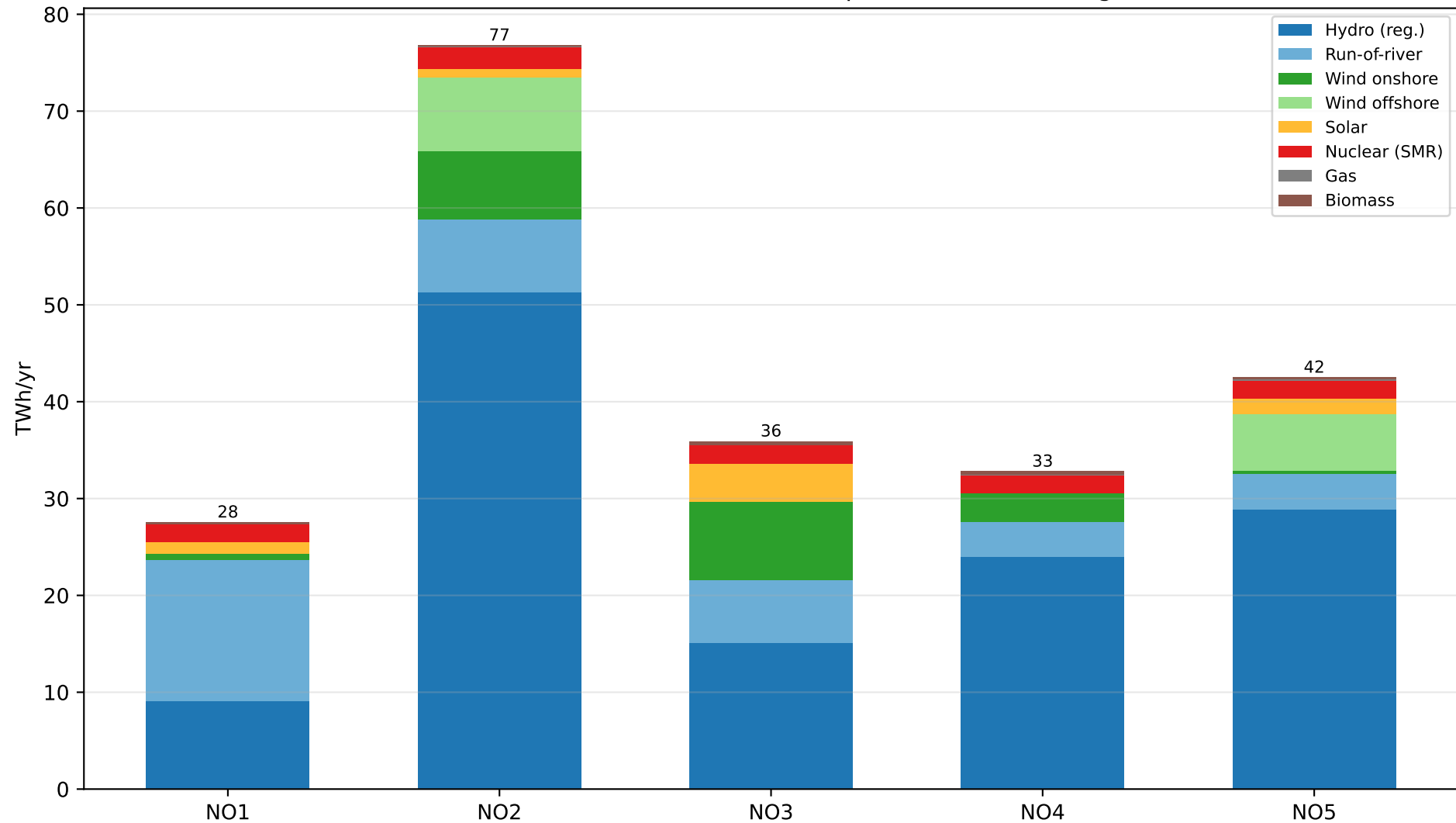
SMR1 (1.5 GW) — Generation Mix per Zone (annual avg)
