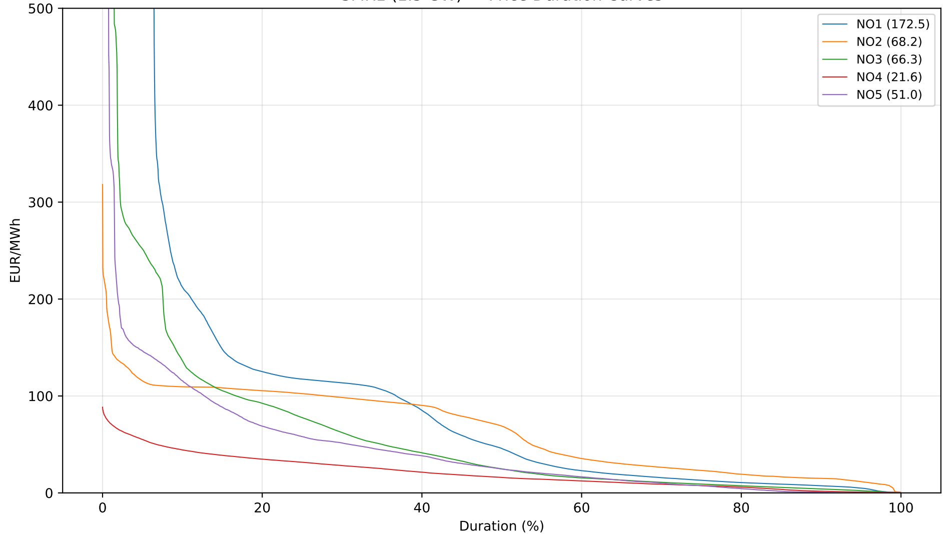
SMR1 (1.5 GW) — Price Duration Curves
