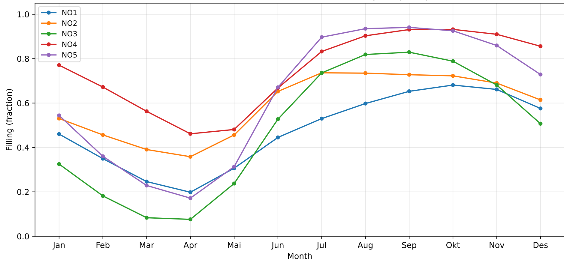
SMR1 (1.5 GW) — Seasonal Reservoir Filling (30-yr avg)
