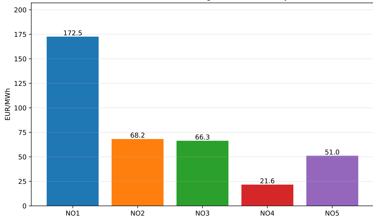
SMR1 (1.5 GW) — Average Zone Prices (30-yr)
