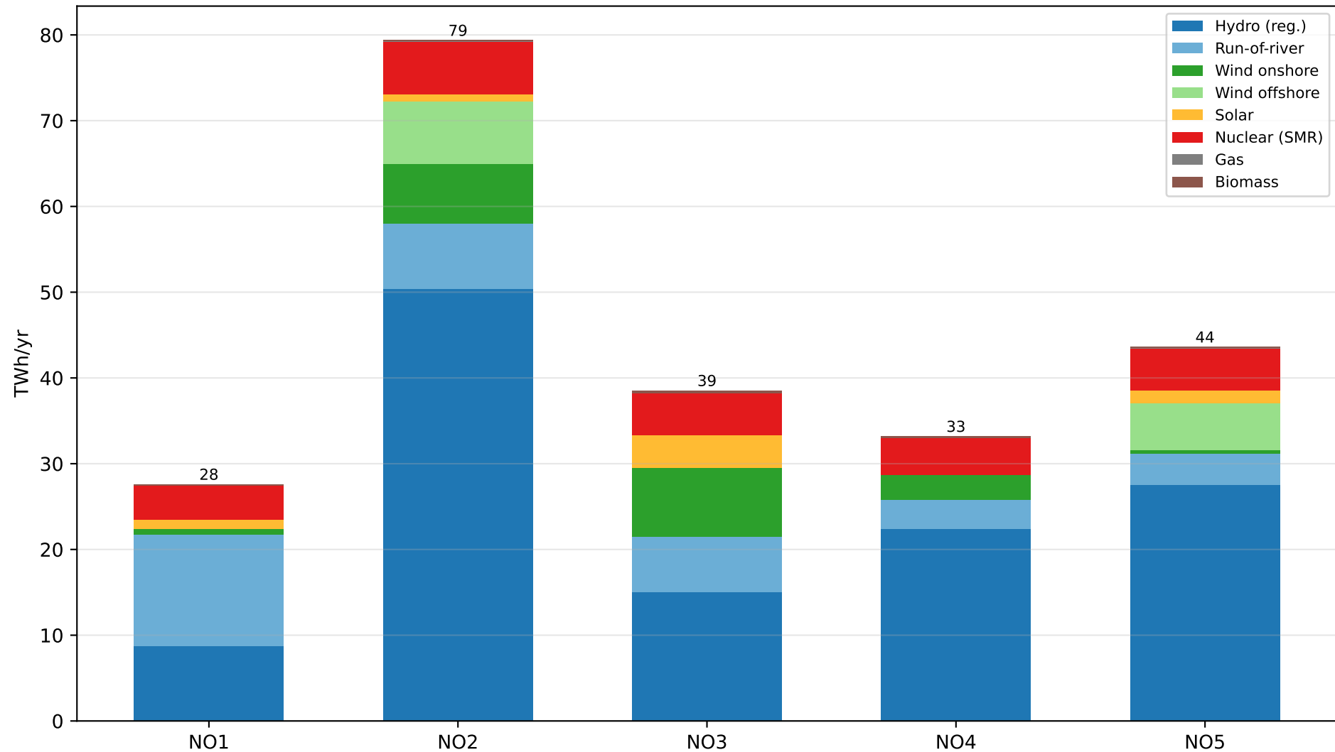
SMR3 (4.5 GW) — Generation Mix per Zone (annual avg)
