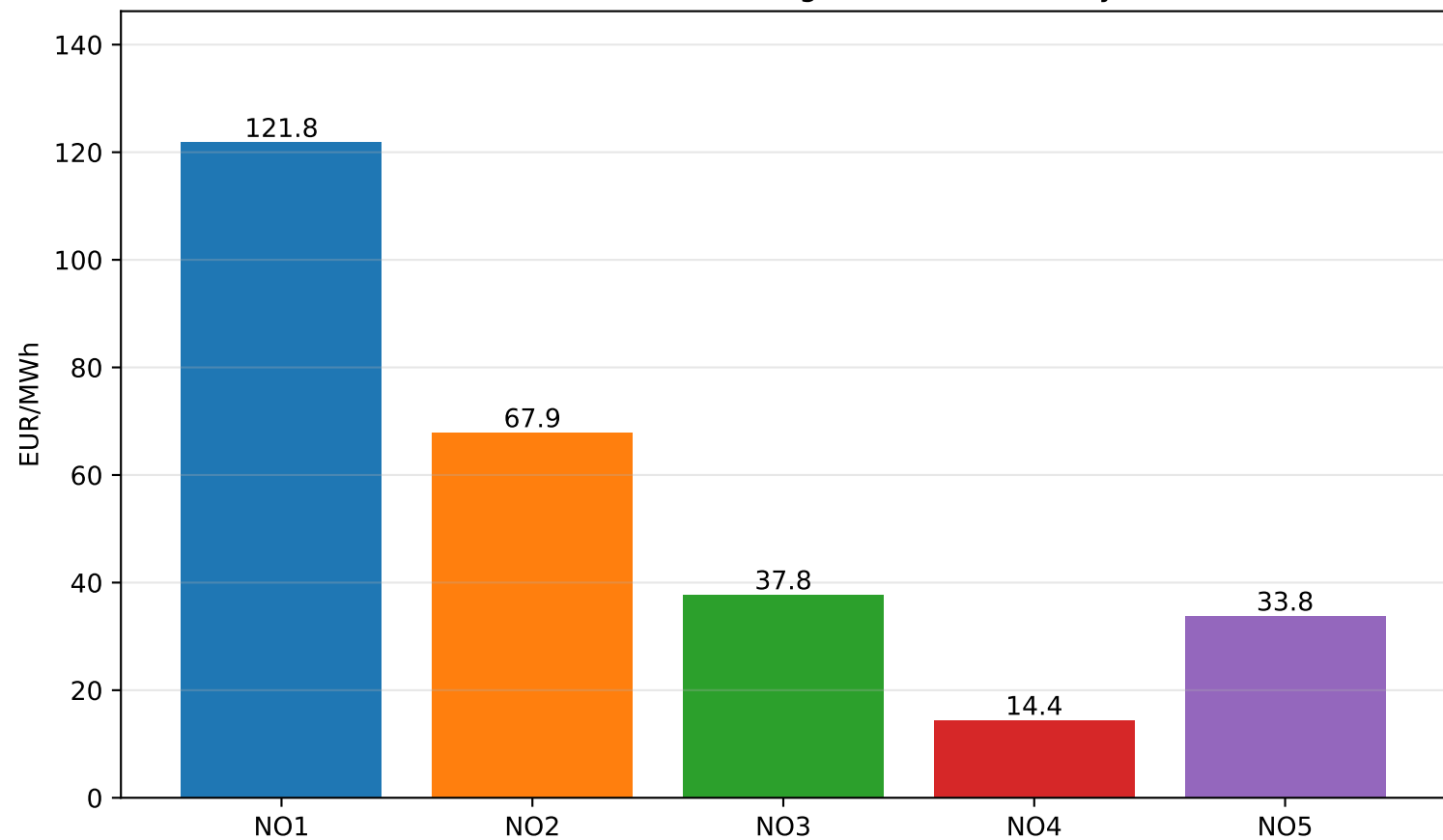
SMR3 (4.5 GW) — Average Zone Prices (30-yr)
