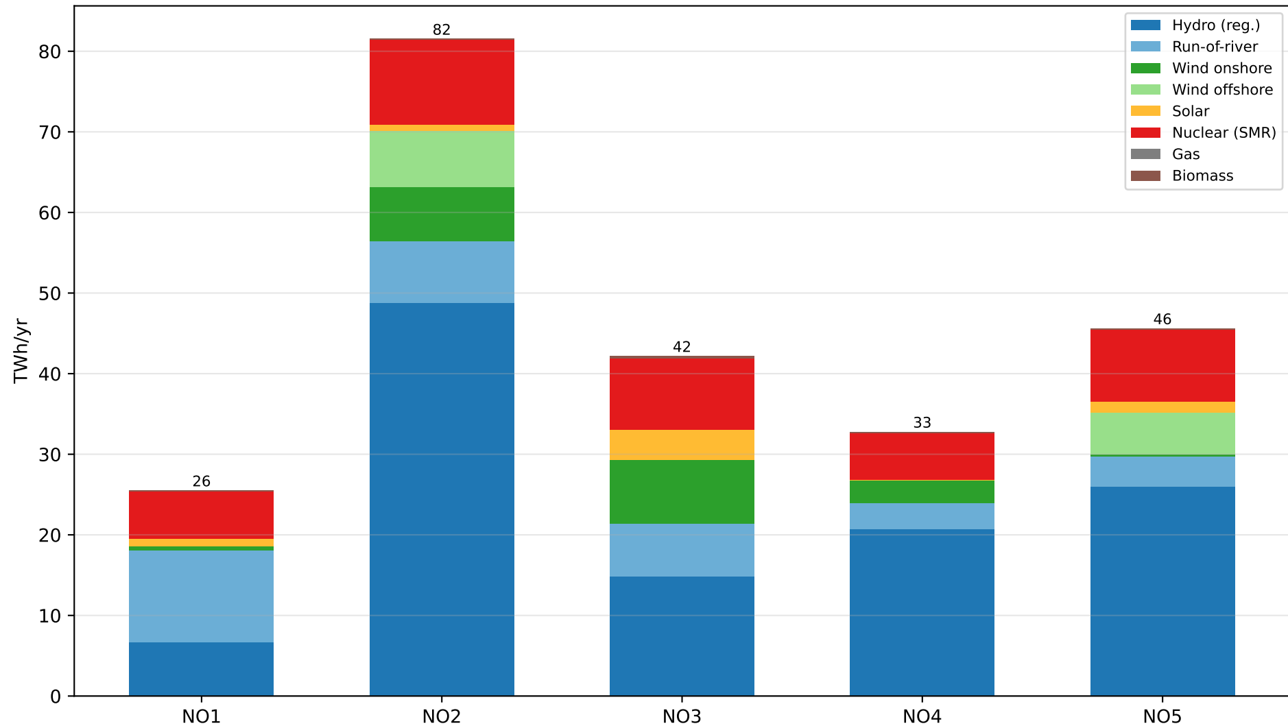
SMR6 (9.0 GW) — Generation Mix per Zone (annual avg)
