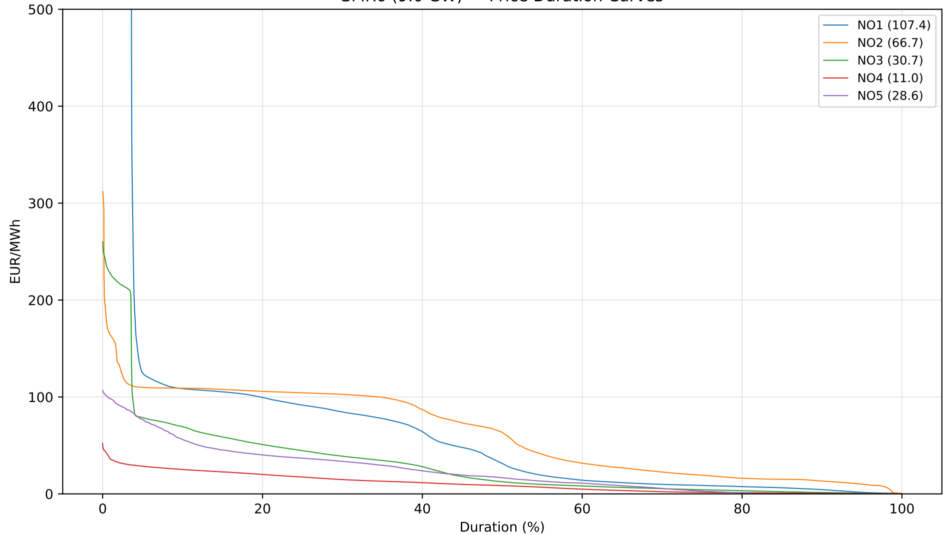
SMR6 (9.0 GW) — Price Duration Curves
