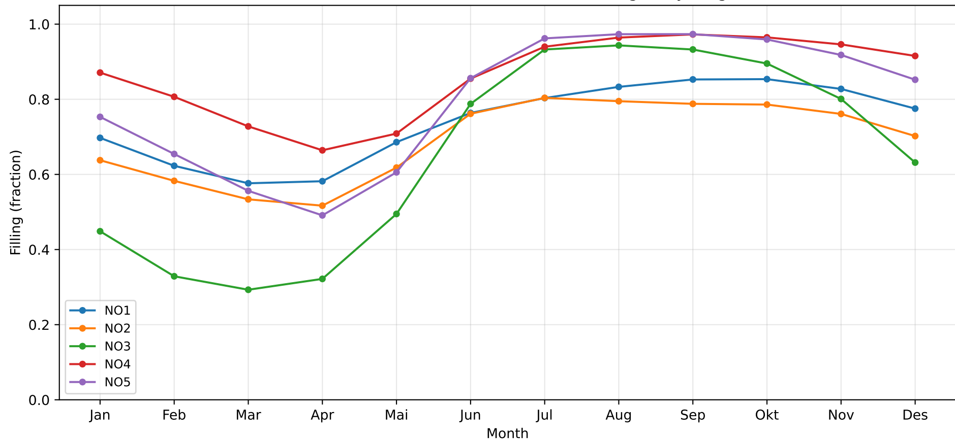
SMR6 (9.0 GW) — Seasonal Reservoir Filling (30-yr avg)
