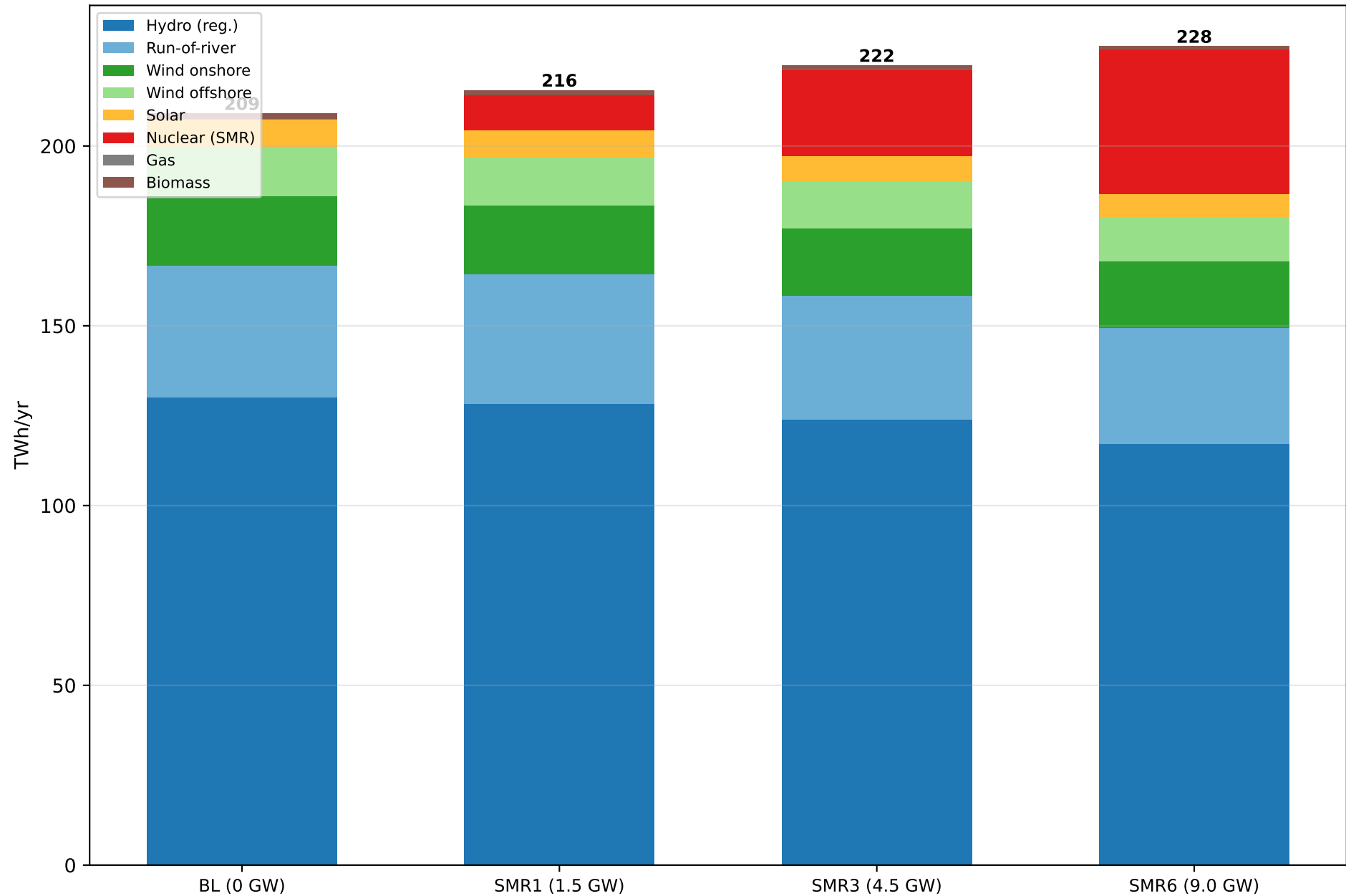
Norway Generation Mix — MD Nuclear Scenarios (annual avg)
