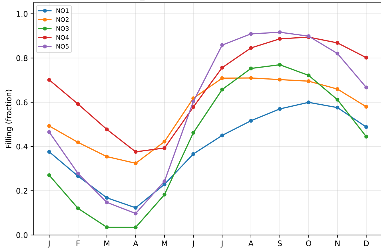
BL_MD — Reservoir Filling by Zone
