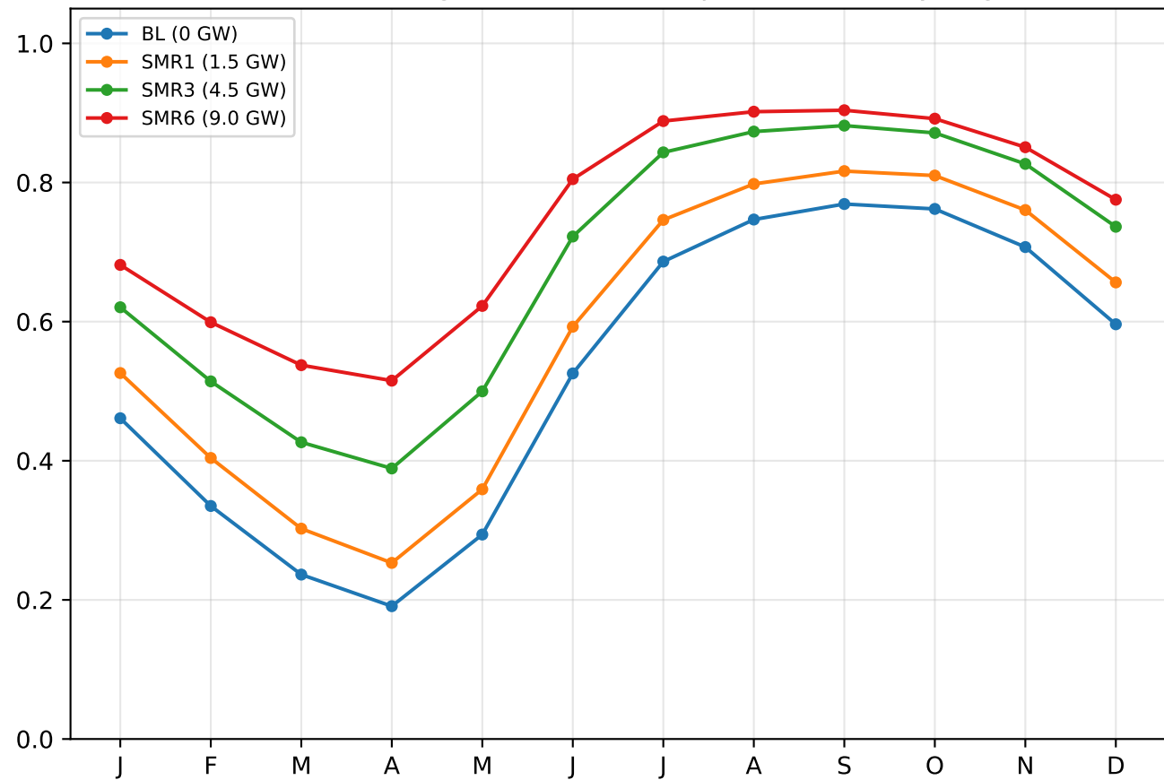
Reservoir Filling — Scenario Comparison (Norway avg)
