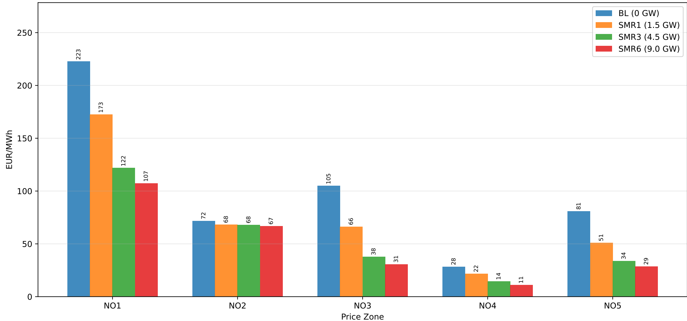
Zone Prices — MD Nuclear Scenarios (30-year average)
