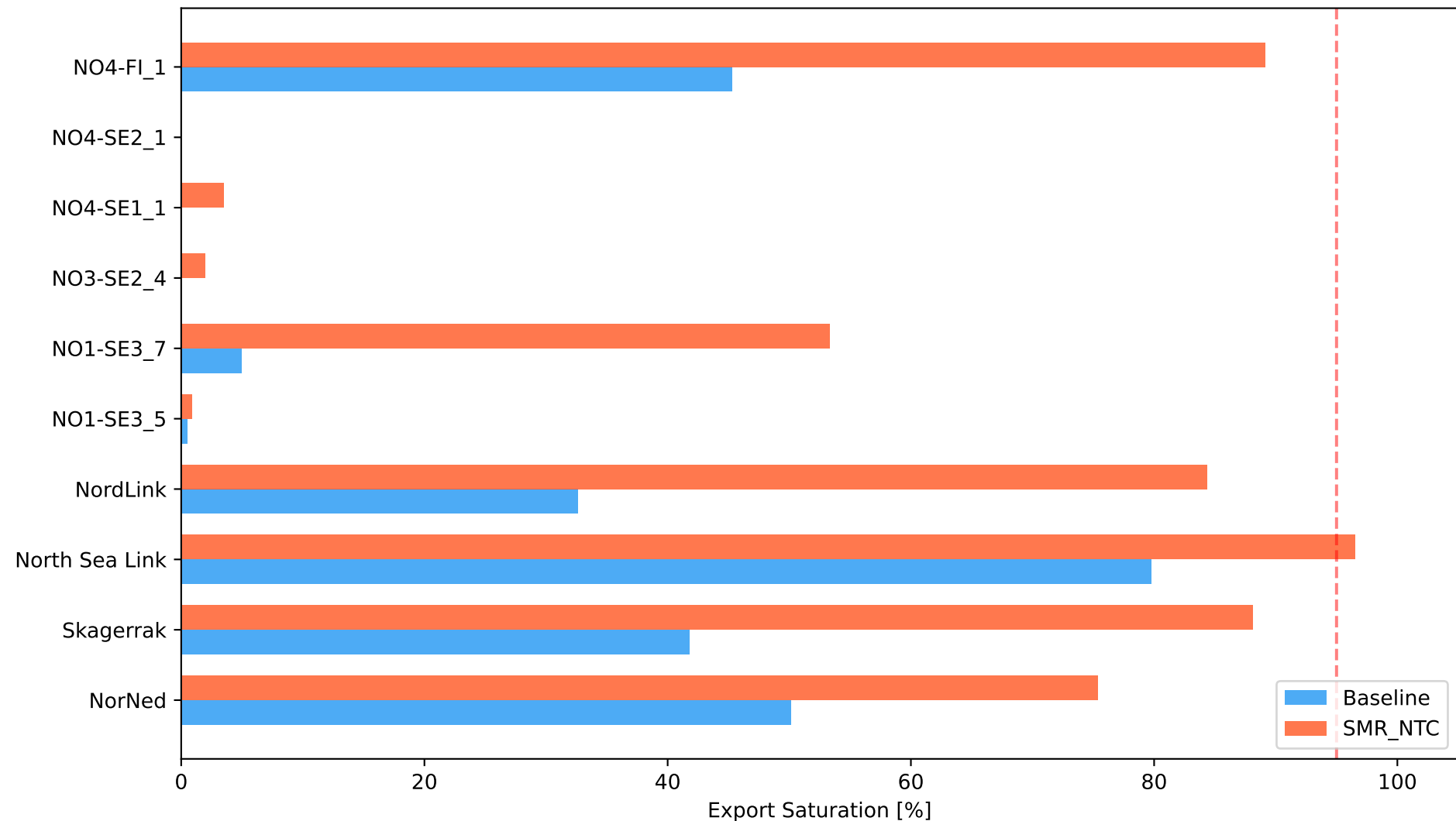
Cable Saturation (>95% NTC) — IC Demand
