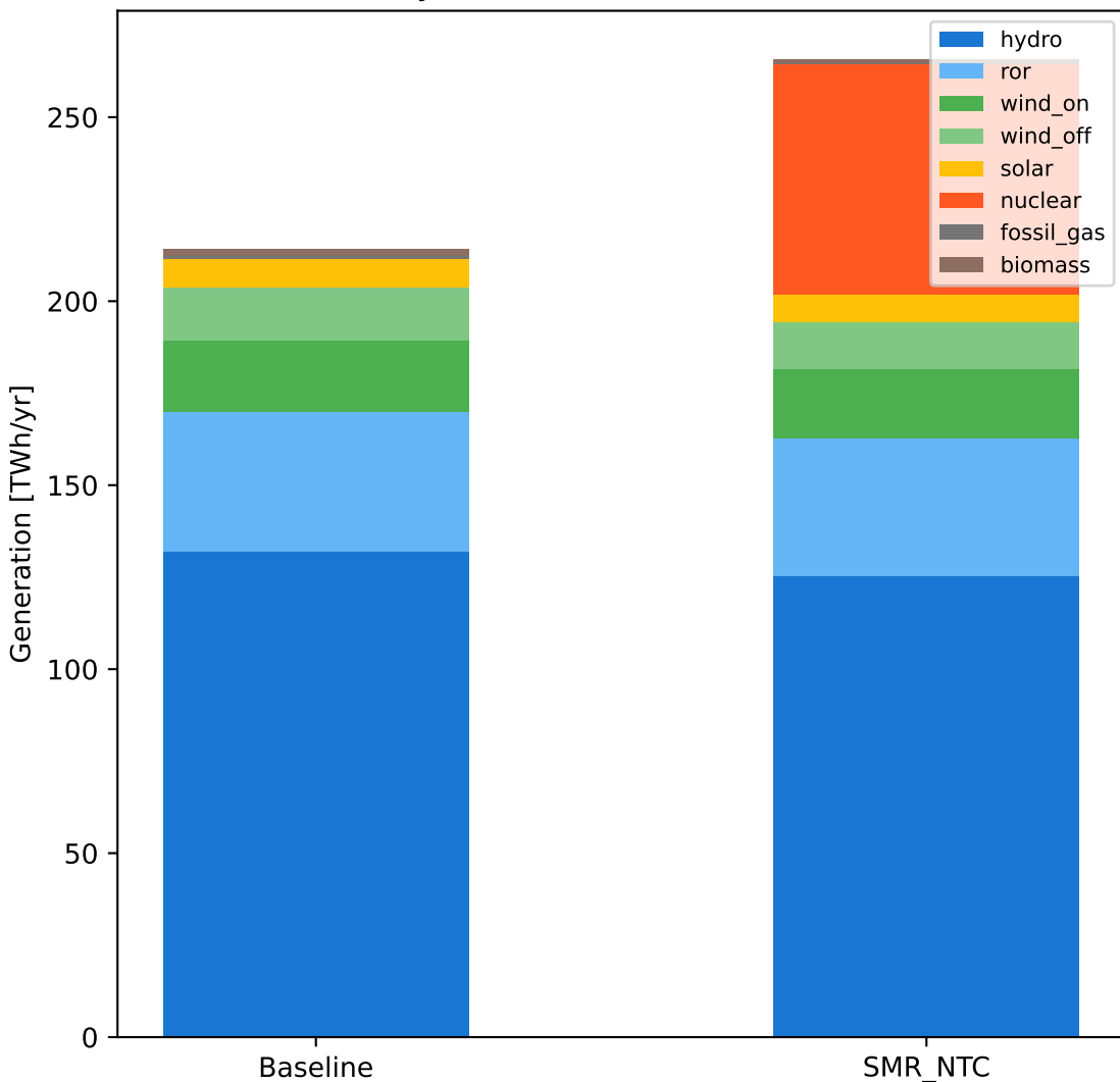
Norway Generation Mix — IC Demand
