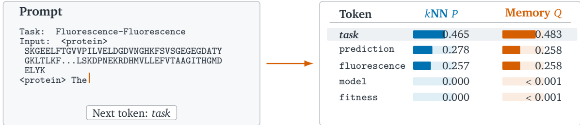
Figure 9 | Protein example. The sequence is abbreviated. The target continuation is highlighted. The right panel compares k NN and memory probabilities for five candidate tokens.
