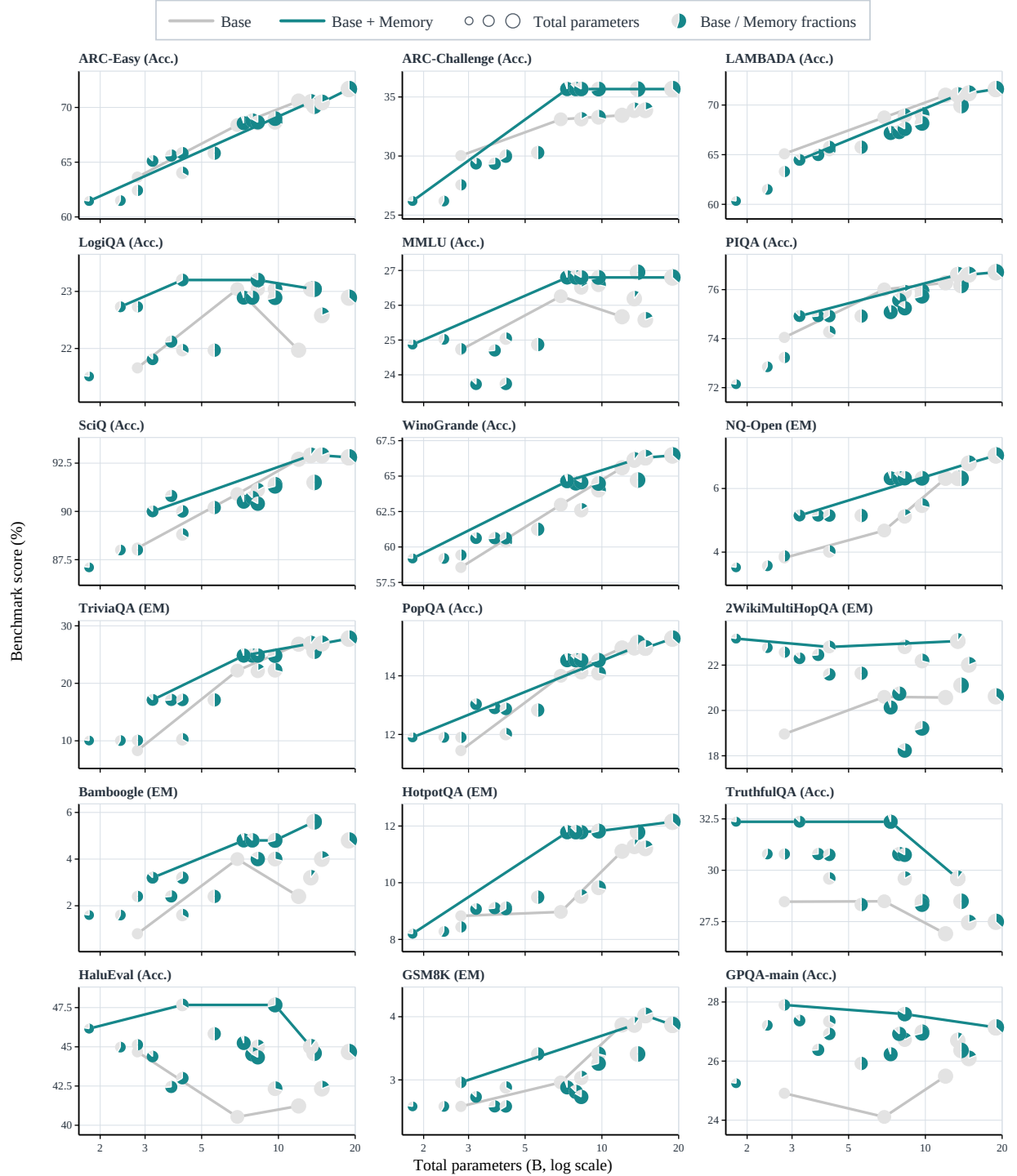
Figure 10 | General memory transfer by task under matched parameter counts and training budgets. Circle area denotes total parameters. Light gray and green denote the Base and Memory fractions, while the lines trace Base and Base + Memory.
