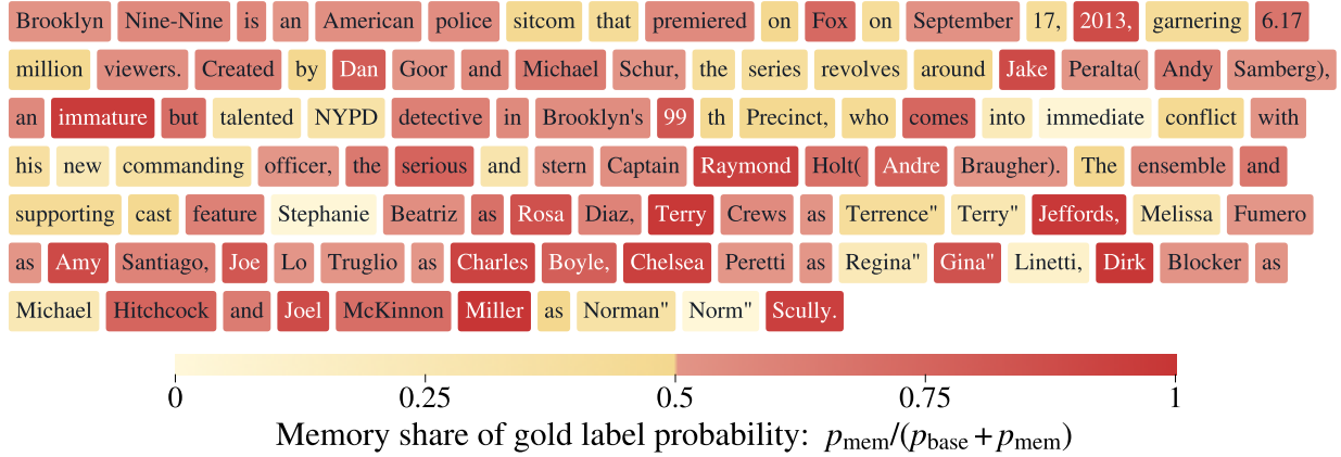
Figure 5 | Memory probability share on the HotpotQA context titled Brooklyn Nine-Nine . Colors encode p_{\text{mem}}/(p_{\text{base}} + p_{\text{mem}}) . Values below 0.5 favor the frozen base model, while values above 0.5 favor the memory model.
