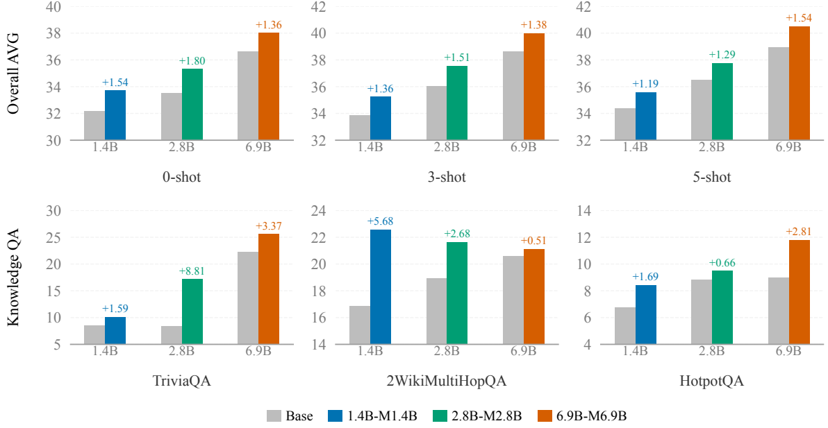
Figure 4 | Top: AVG over the same 14 tasks under zero-shot, three-shot, and five-shot settings. Bottom: Zero-shot results on TriviaQA, 2WikiMultiHopQA, and HotpotQA. Gray bars denote frozen backbones. The notation x.xB-Mx.xB represents an x.xB backbone paired with an x.xB memory.
