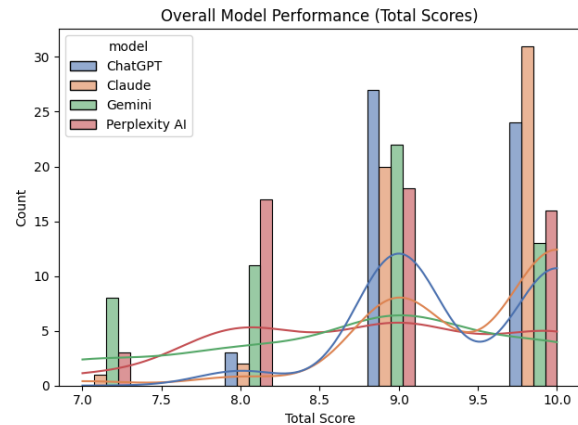
Figure 1: Distribution of total scores across models.
