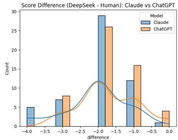
Figure 3: Distribution of score differences between AI-based and human evaluation.
