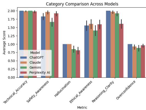
Figure 2: Average scores across evaluation metrics.
