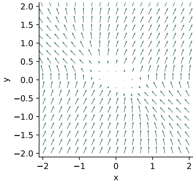
Exact: gradient of a polynomial
