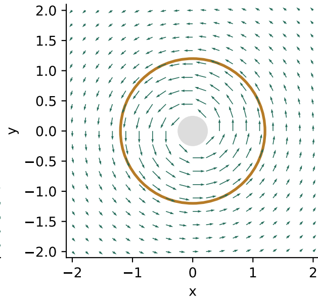
Vortex: remove the origin
