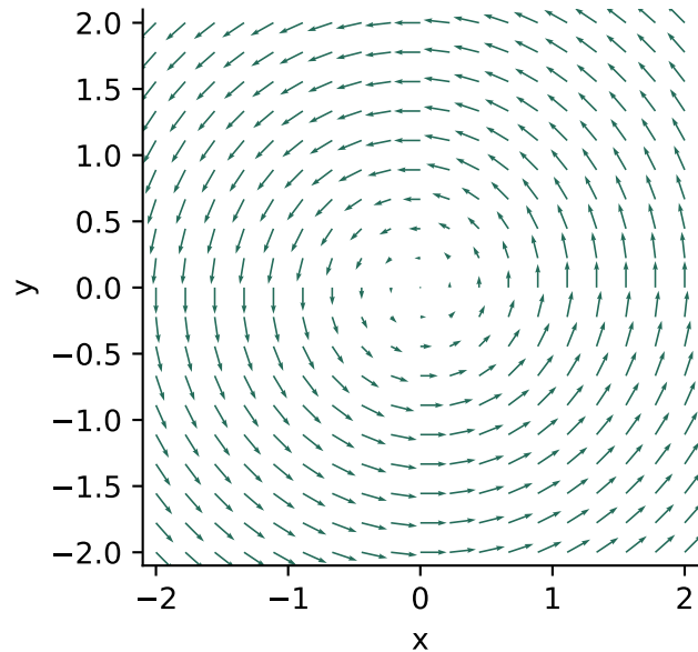
Rotation: mixed partials differ
