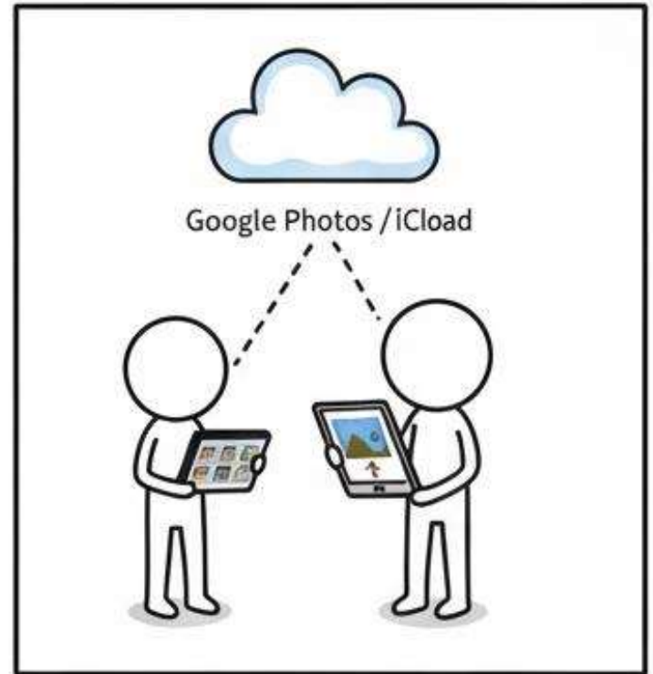
CLOUD STORAGE
