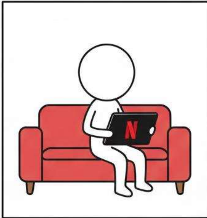
STREAMING
